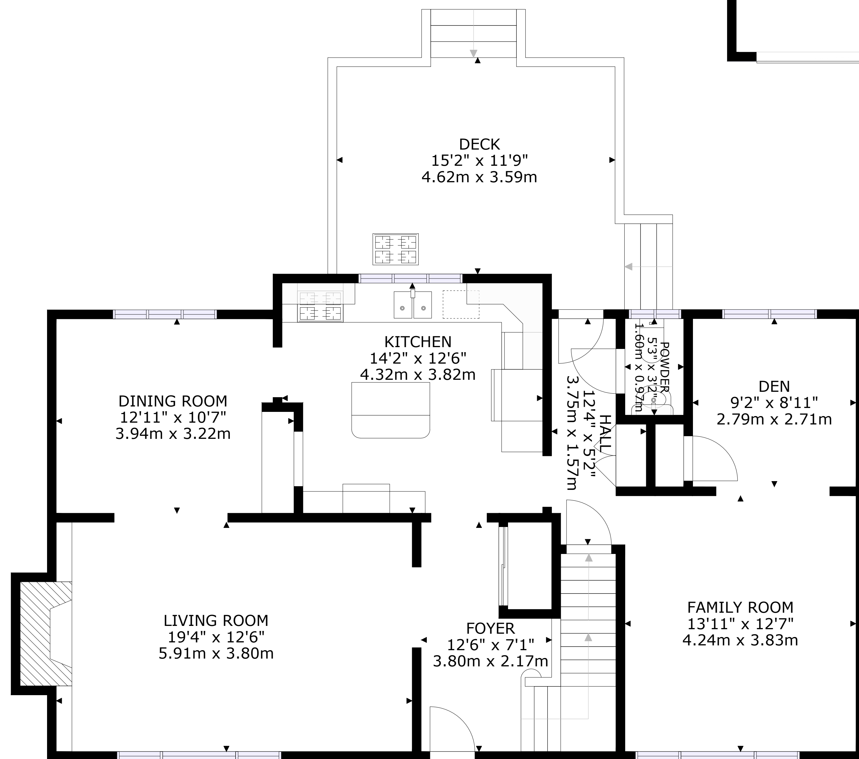
FLOOR 2
