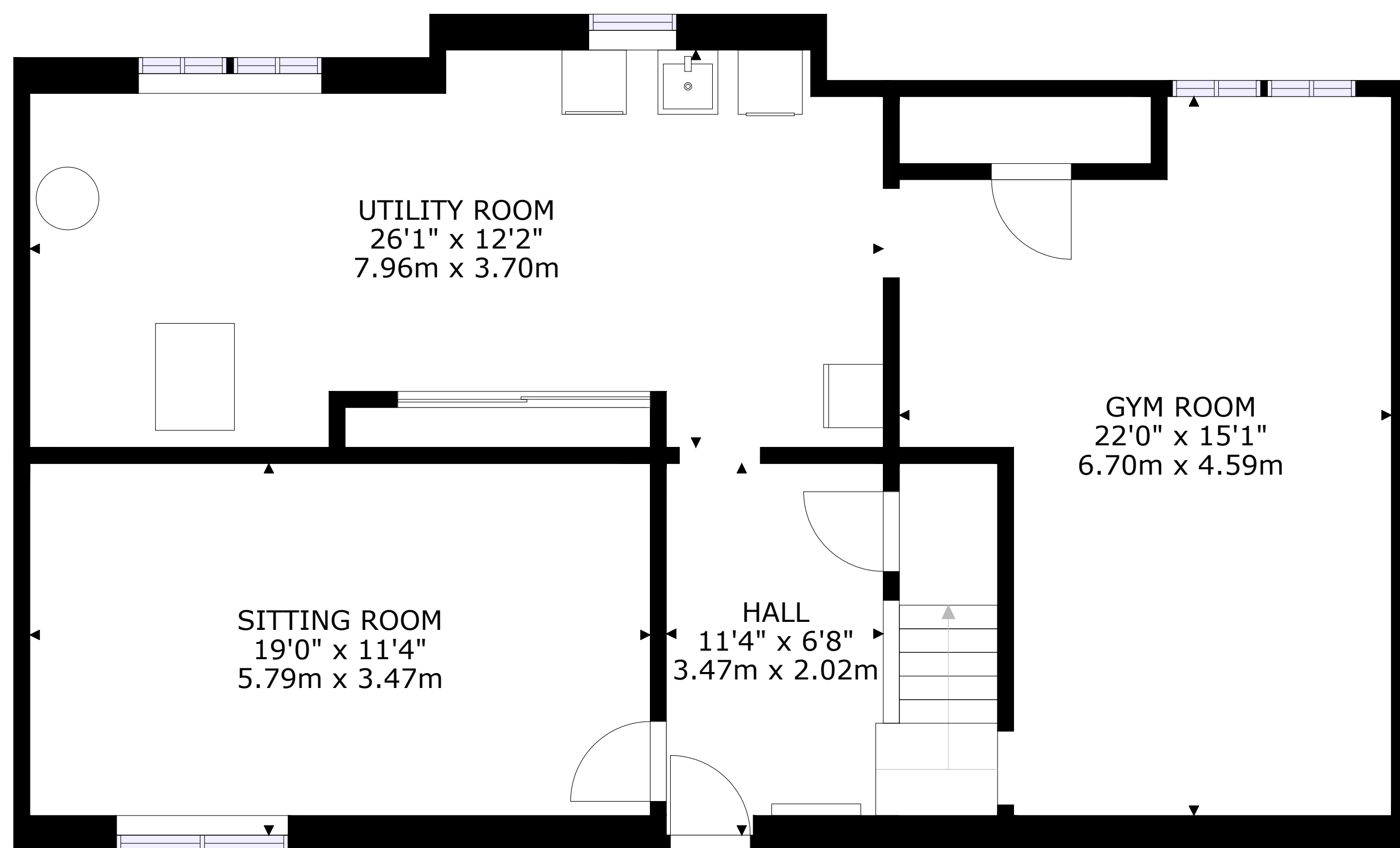
FLOOR 1
