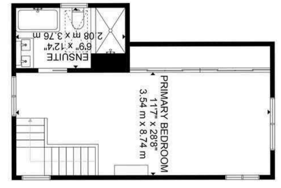
Main House Second Floor
