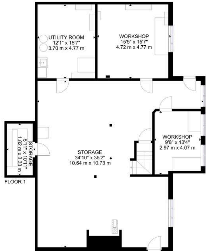
Basement
