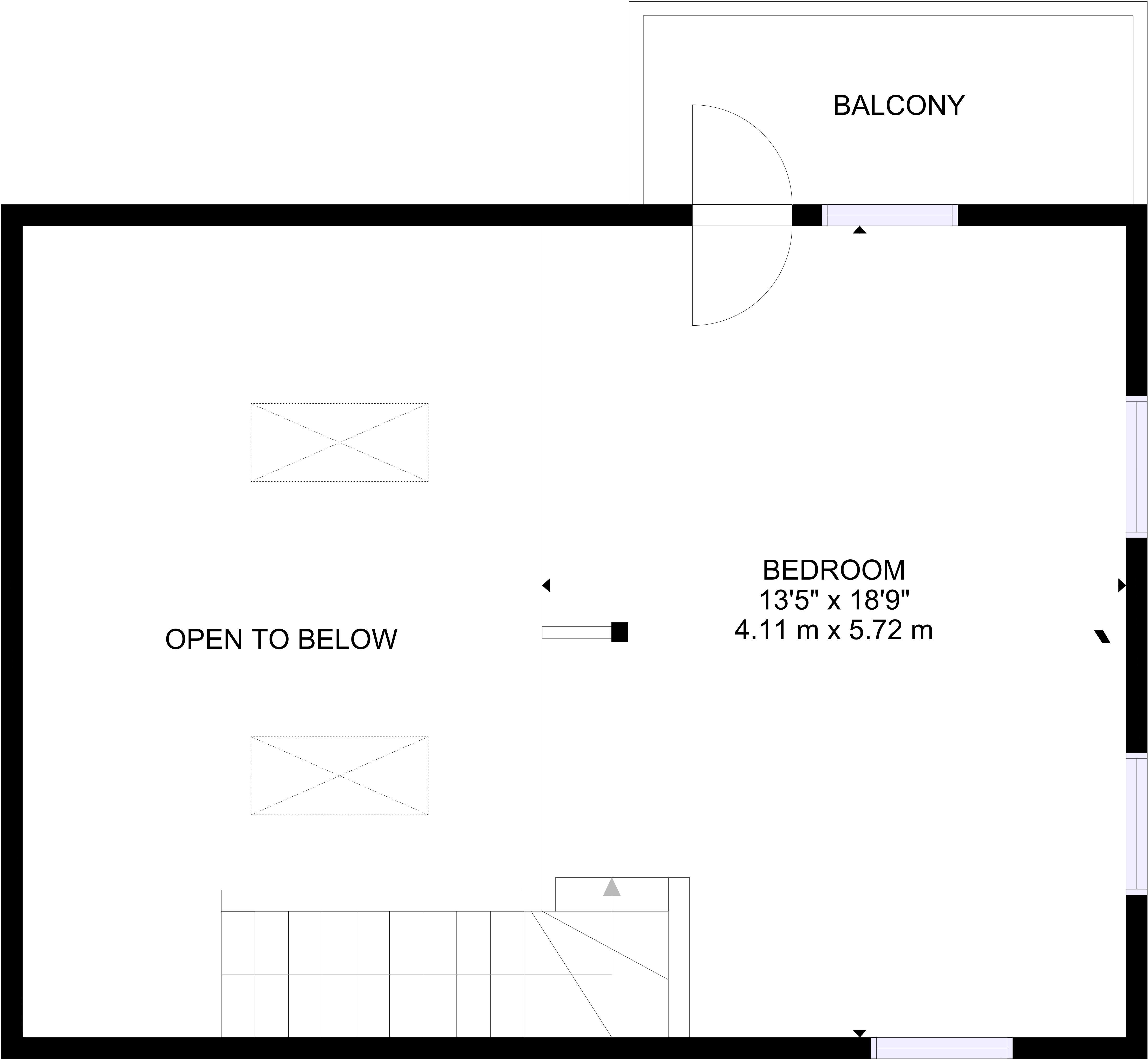
FLOOR 2
