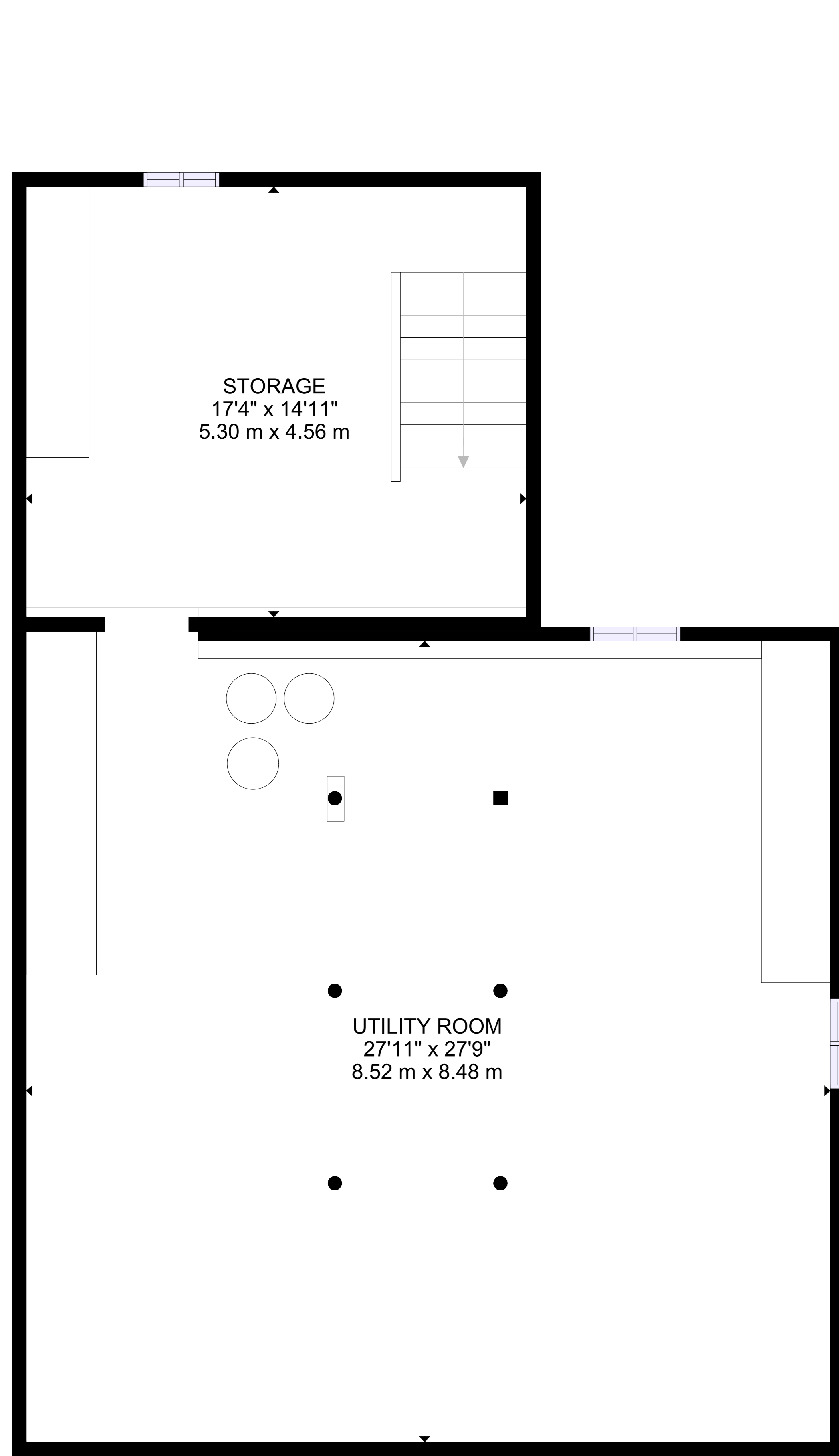
FLOOR 1
