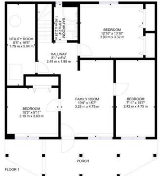
BASEMENT
