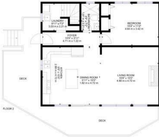
MAIN LEVEL
