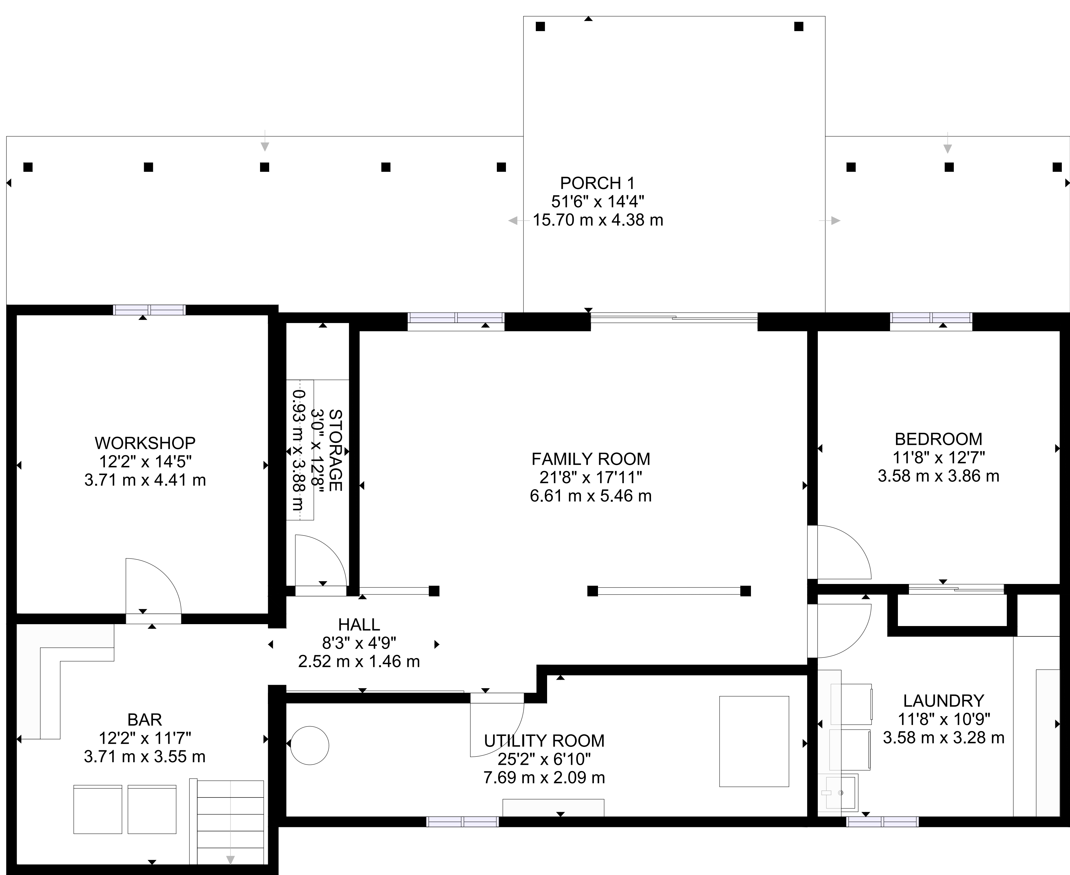
FLOOR 1
